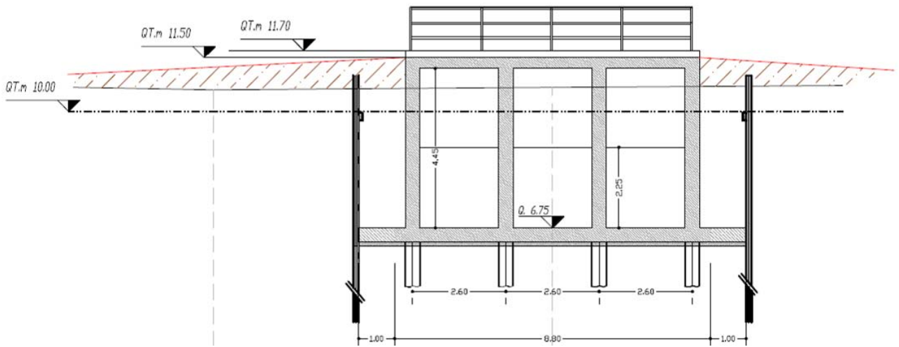
Picture 5 - Transverse profile of the final design
