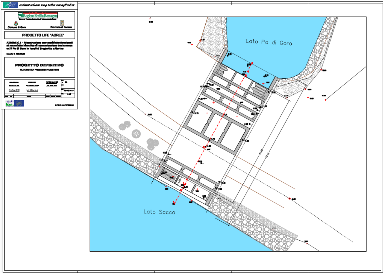
Picture 3 - Plan view of the hydraulic structure (n. 3 bulkheads)
